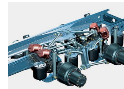
Construction air suspension at the rear axle with ECAS electronic level control.
