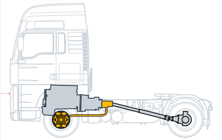
MAN HydroDrive® operating principle.
